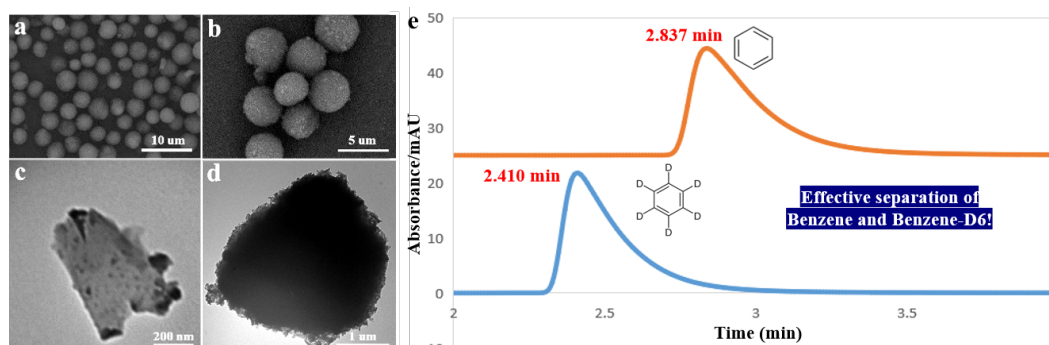
Figure 1. SEM images of (a) \text{SiO}_2\cdot\text{NH}_2 and (b) graphene-decorated \text{SiO}_2\cdot\text{NH}_2\cdot\text{PFPA}\cdot\text{NHS} ; TEM images of (c) graphene nanosheets and (d) graphene-decorated \text{SiO}_2\cdot\text{NH}_2\cdot\text{PFPA}\cdot\text{NHS} ; (e) chromatograms of benzene and benzene-D 6 with hexane as the mobile phase.
